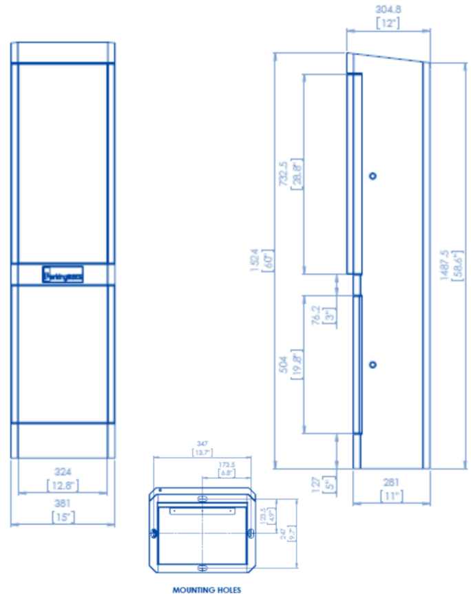
MOUNTING HOLES
